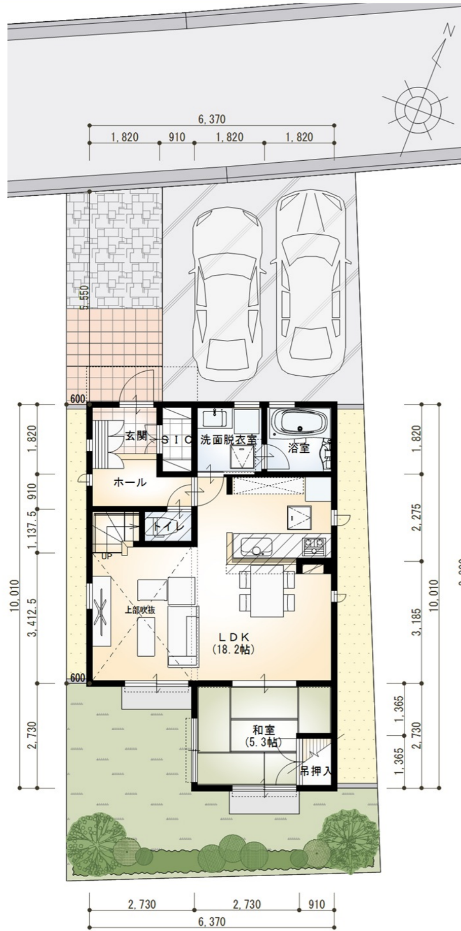
1st Floor
